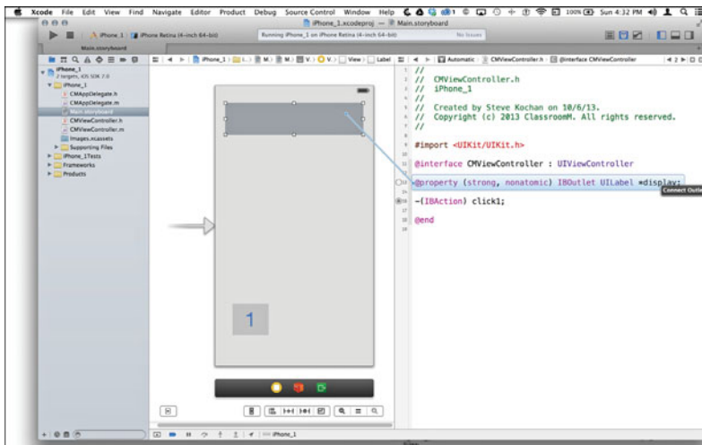
Figure 21.16 Connecting an outlet variable
