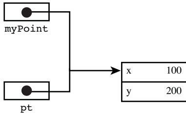
Figure 8.6 Passing the rectangle's origin to the method
