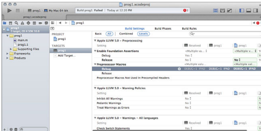
Figure 12.1 Defining the preprocessor identifier IPAD
