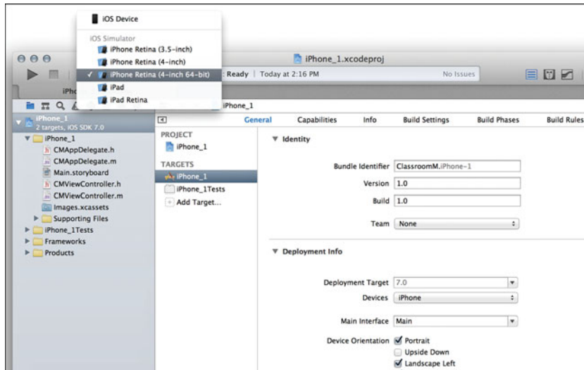
Figure 21.7 Selecting the iPhone simulator
